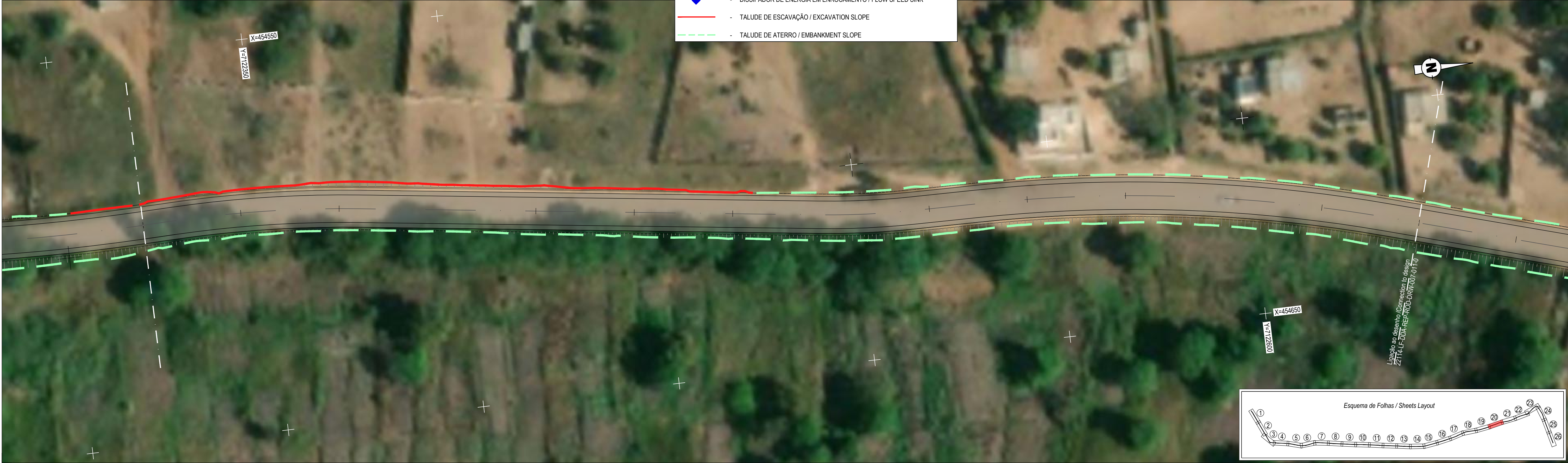
DRENAGEM PLUVIAL / STORMWATER DRAINAGE PLANTA / PLAN Access B: km 5+725 - km 6+050 Escala / Scale 1:500
