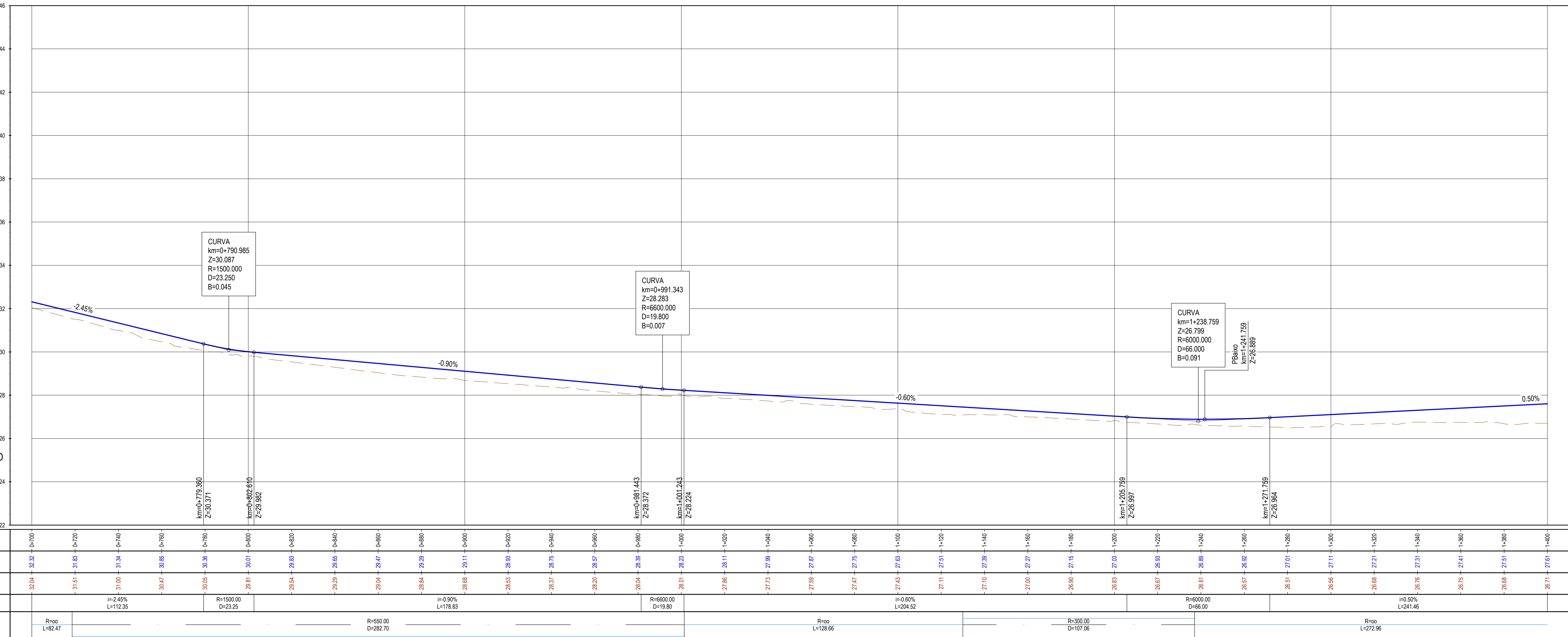
ACESSO B / ACCESS B ROAD PERFIL LONGITUDINAL / PROFILE Escala / Scale H=1:1000; V=1:100
